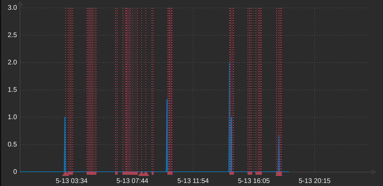
Queue size
