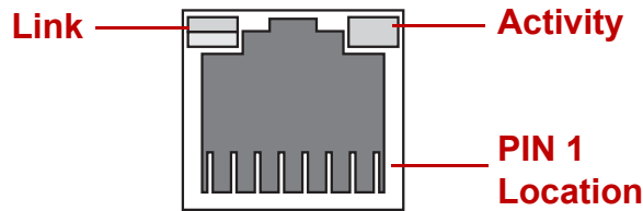
Figure 1-13. GbE RJ45 Management Port
