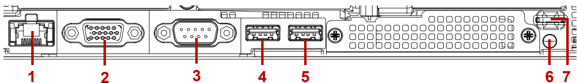
Figure 1-7. System Rear I/O
